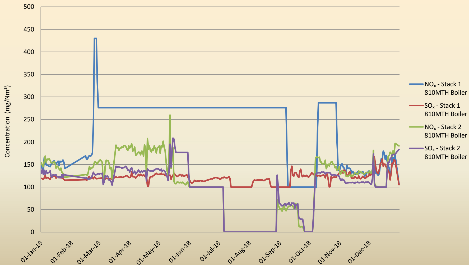
Annual Emission Trend of Gaseous in M/s. Jaiprakash Power Vntures Ltd., Dist. Sagar (M.P.)
